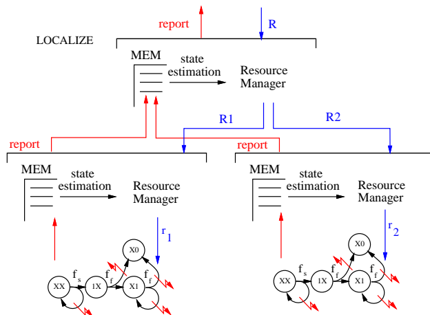
Figure 5: LOCALIZE - A Physical Schema for localizing features in space.
